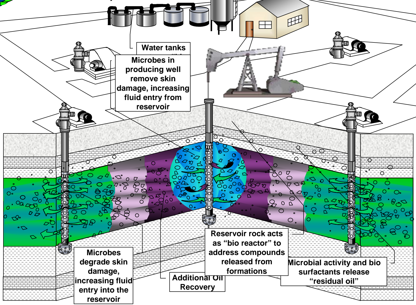
Single 5-Spot Pattern
